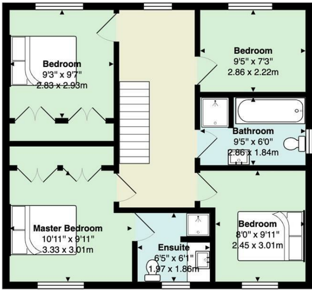
42a Craiglee Drive Total Area: 1261 ft² ... 117.2 m² All measurements are approximate and for display purposes only
